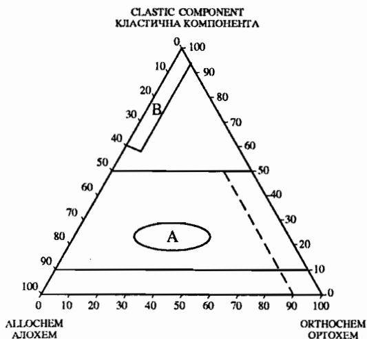
Fig. 4. Three-component diagram of clastic component-allochem-ortochem (Folk, 1974) with field of investigated limestone fragments. A - carbonate rocks; B - terrigenic sediments.
