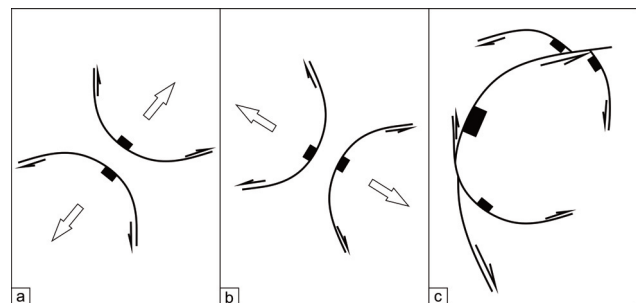
Fig. 7. Sketch of the mechanism of strain partitioning between coeval faults with different kinematics. a) Half grabens formed by NE–SW extension. b) Half grabens formed by NW–SE extension.
