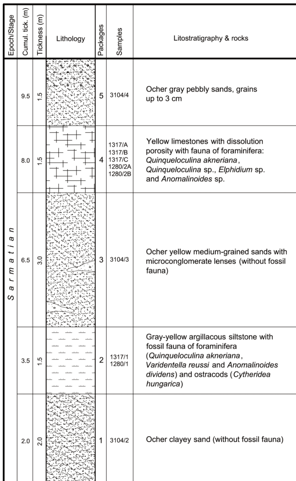
Fig. 7. Sarmatian stratigraphic column of the vicinity of Bogava and the Kamenovo Formation.
