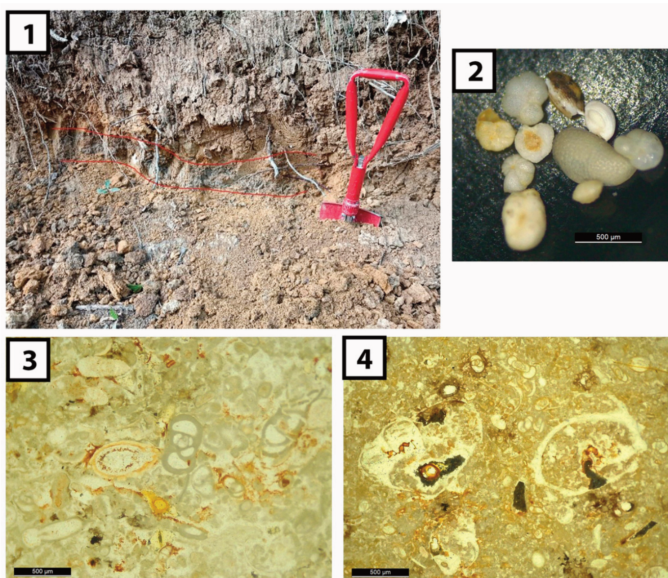
Fig. 10. Sarmatian gray-yellow argillaceous siltstone (marked with red lines, 1), with extracted microfauna of foraminifera and ostracods ( Quinqueloculina akneriana D'ORBIGNY, Anomalinoidea dividens LUCZKOWSKA, Cytheridea hungarica (ZALANYI) etc., 2); and thin-sections from Sarmatian yellow limestone with cross sections of foraminifera (3, 4) and microgastropods (4).
