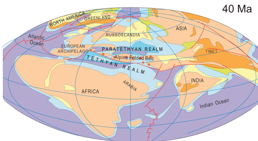
Fig. 1. Map depicting the paleogeography of Eurasia and nearby territories in the second half of the Eocene epoch of the Paleogene period (40 Ma) (POPOV et al., 2004). Legend shown in Fig. 3.
