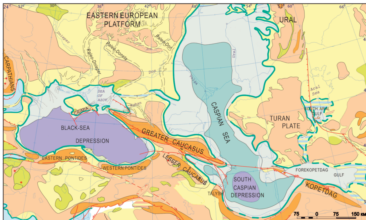
Fig. 7. Paleogeographic map of the Eastern Paratethys in the Pliocene-Early Pleistocene (2.2–2.6 Ma) (modified after POPOV et al., 2004).
