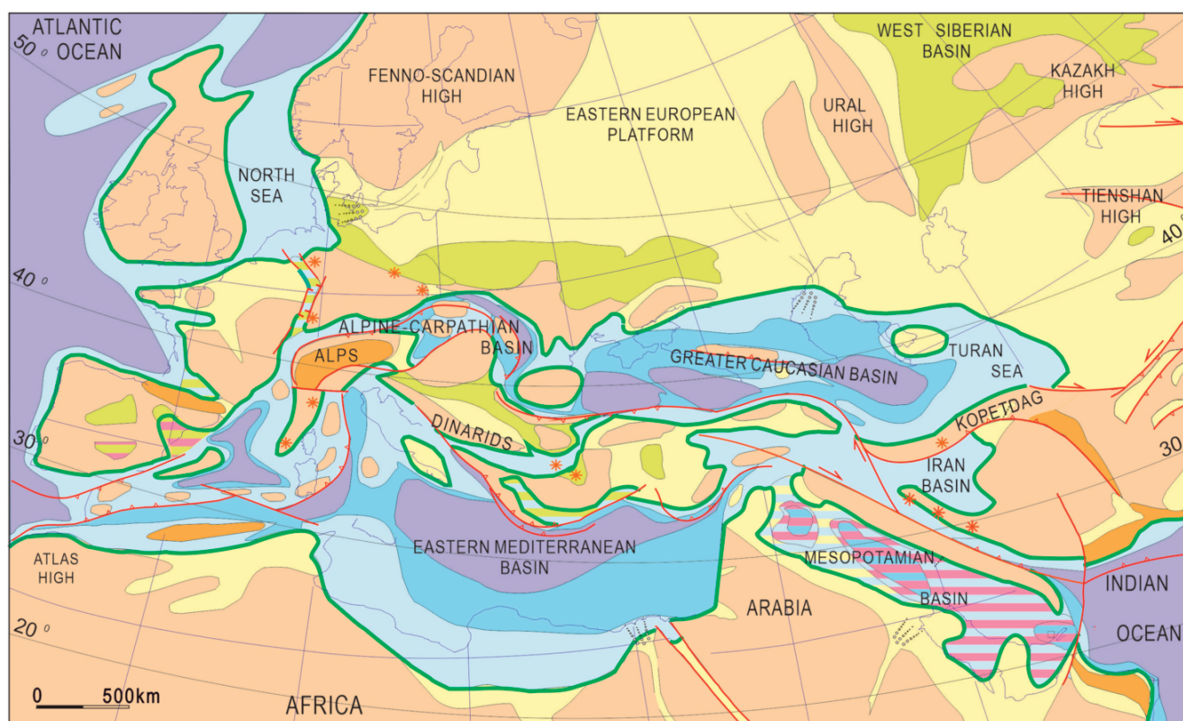
Fig. 5. Paleogeographic map of the Western Eurasia in the first half of the Early Miocene (18–20.5 Ma) (after Popov et al., 2004).
