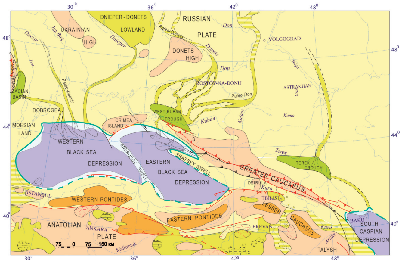
Fig. 10. Paleogeographic map of the Eastern Paratethys during the terminal Sarmatian regression, 7.6 Ma.
