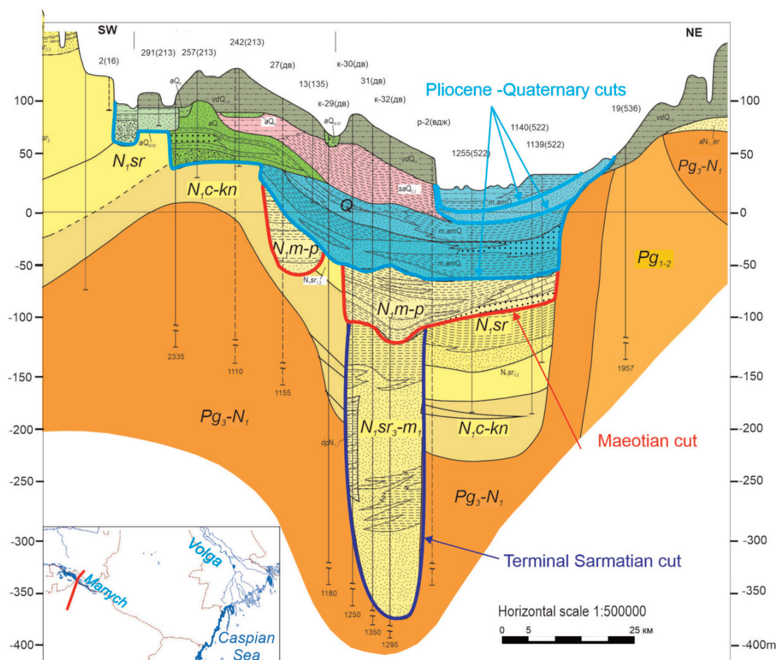
Fig. 9. Two generations of the paleo-Don River Neogene incisions in the Manych area as a result of falls of the erosion basis at the end of Sarmatian and at the end of Maeotian–Pontian, filled with marine sediments of subsequent transgressions (TIMOKHIN et al., 2009).
