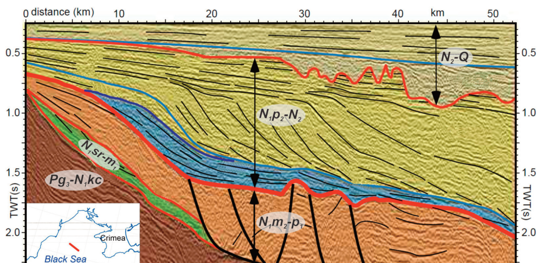
Fig. 8. Seismic section of the western (Romanian) shelf of the Black Sea (MUNTEANU et al., 2012). The boundaries of the unconformities which reflect erosion of the underlying rocks are marked by red lines. Indices show the rock age: Pg_3-N_1kc – Oligocene–Miocene; N_1sr-m_1 – Sarmatian–Lower Maeotian; N_1m_2-p_1 – Upper Maeotian–Lower Pontian; N_1p_2-N_2 – Upper Pontian–Pliocene; N_2-Q – Pliocene–Quaternary. The inset on the lower left shows its location.
