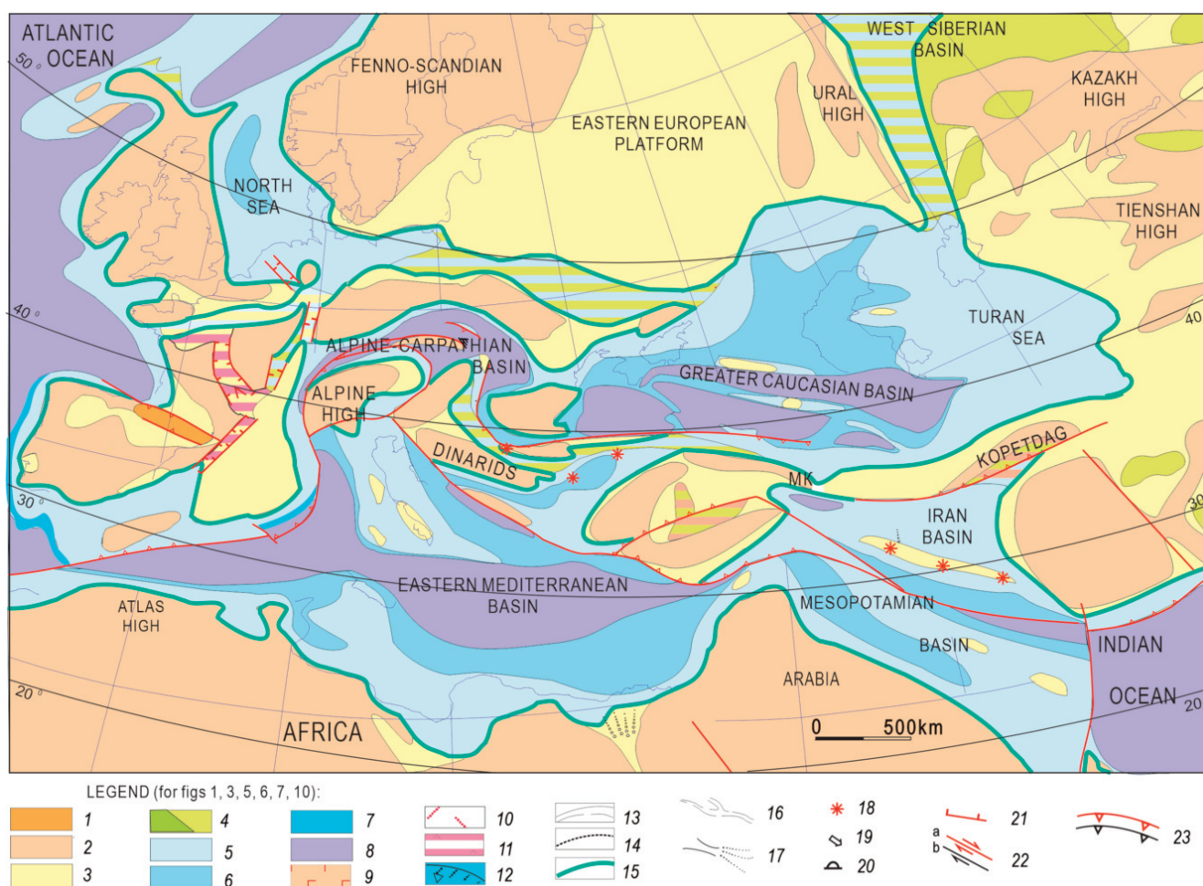
Fig. 3. Paleogeographic map of the Western Eurasia in the first half of the Early Oligocene (32–34 Ma) (after Popov et al., 2004, modified). Legend (for all paleogeographic maps): 1. mountains; 2. high lands; 3. low lands; 4. lagoons and lakes; 5. shallow shelf; 6. deep shelf; 7. depressions; 8. bathyal; 9. intrusive massifs; 10. acidic extrusives; 11. salt marches and lagoons; 12. slopes of depressions; 13. paleogeographic boundaries; 14. facial boundaries; 15. sea\continental boundary; 16. river valleys; 17. river deltas, fans; 18. volcanoes; 19. sediment source; 20. bioherms; 21. faults; 22. thrusts (active - red, subsequent - black); 23. shifts active and subsequent.
