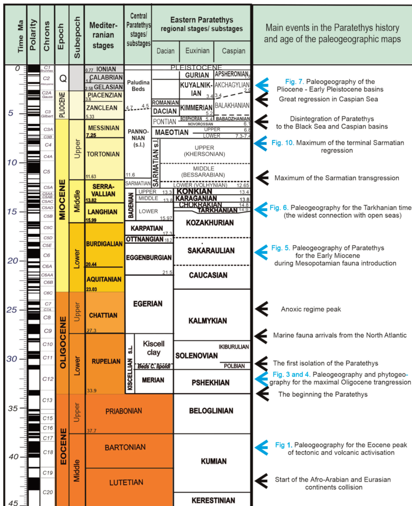
Fig. 2. Stratigraphic scales of the Mediterranean, Central and Eastern Paratethys (according to PALCU et al., 2017, 2019; GRADSTEIN, 2020; Popov et al., 2022) and the main events of the Paratethys evolution. The blue arrows show the stratigraphic levels for which the paleogeographic maps are given.
