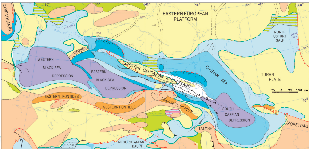
Fig. 6. Paleogeographic map of the Eastern Paratethys in the Middle Miocene (Tarkhanian) (14.8–14.9 Ma) (modified after POPOV & PATINA, 2023).
